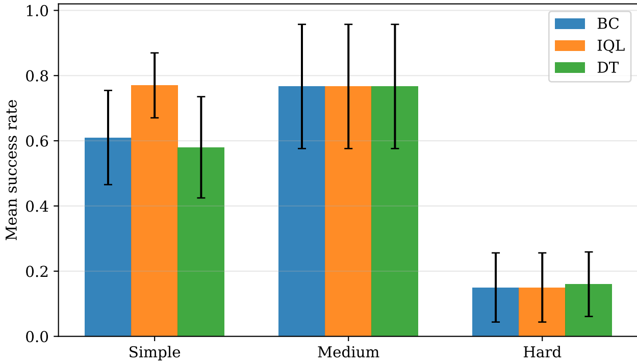
Performance by Task Tier (N=50)
