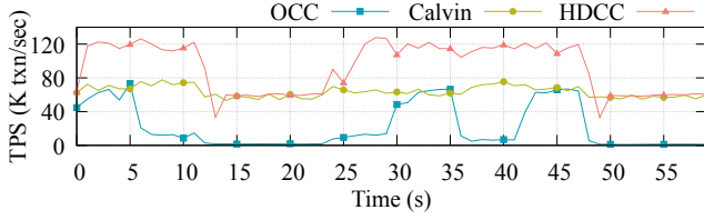
Figure 12: Effect of dynamic workload (YCSB)
