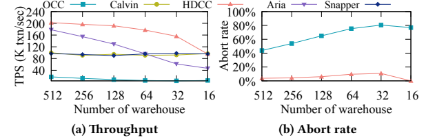
Figure 17: Effect of the contention level (TPC-C)
