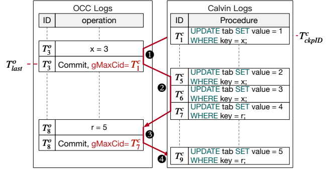
Figure 8: Two-log-interleaving mechanism
