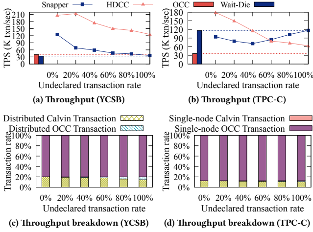
Figure 19: Effect of undeclared transaction rate
