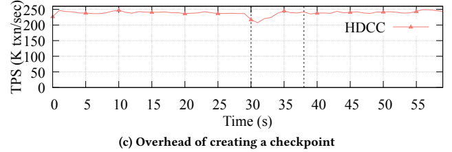
Figure 13: Scalability, overhead of logging, and checkpoint creation (YCSB)
