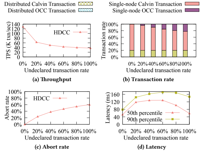
Figure 10: The overhead analysis of O2
