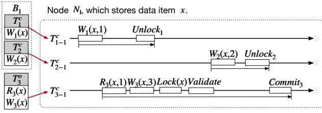
Figure 4: A running example of incorrect local schedule
