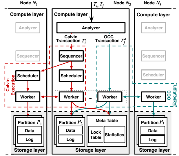
Figure 3: An overview of HDCC
