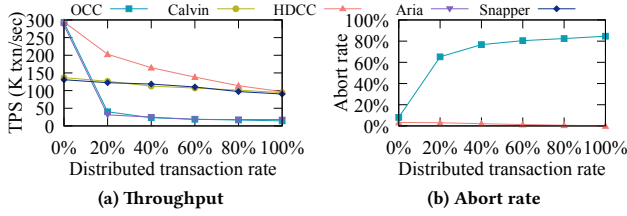
Figure 14: Effect of distributed transaction rate (YCSB)
