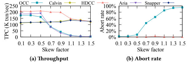
Figure 16: Effect of the contention level (YCSB)
