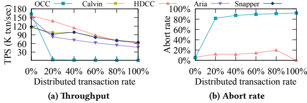
Figure 15: Effect of distributed transaction rate (TPC-C)
