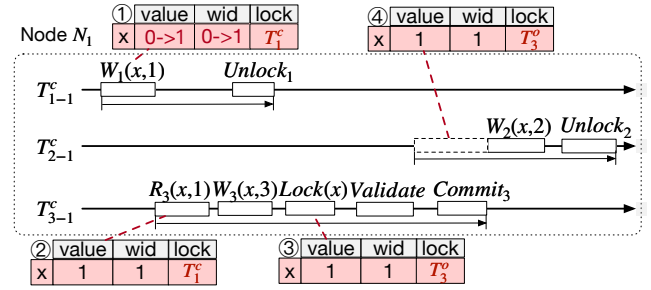
Figure 5: A running example of lock-sharing mechanism
