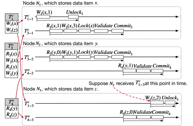
Figure 6: A running example of incorrect global schedule
