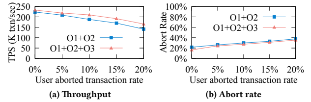
Figure 11: The overhead analysis of O3
