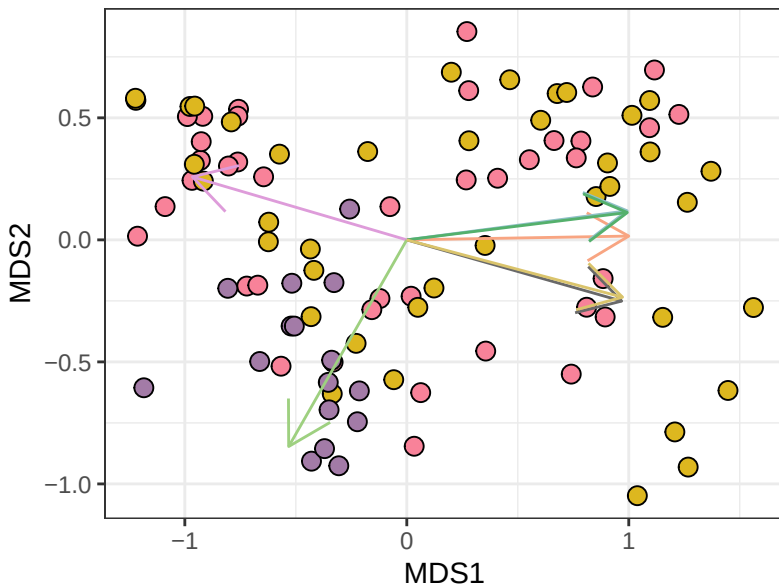
Coarse-Scale NMDS (MDS1 v MDS2)
