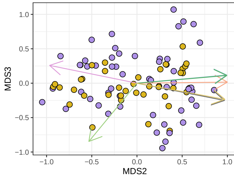
Coarse-Scale NMDS (MDS2 v MDS3)
