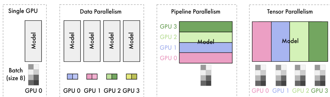
Figure 8.8 – Illustration of the different model parallelism techniques
