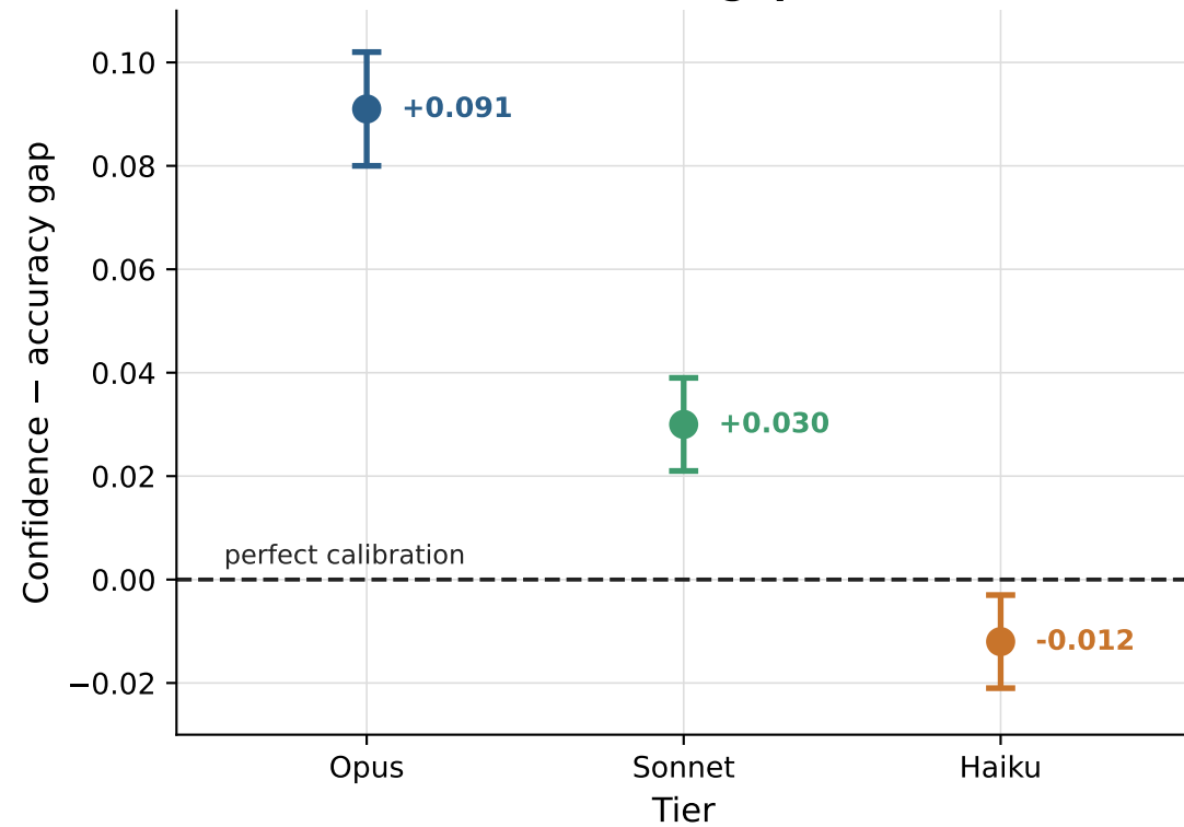
Overconfidence gap (95% CI)
