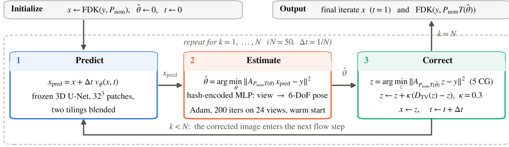
Figure 2: Overview of the proposed method. (a) The geometry bridge used for training: each panel is an FDK reconstruction of the same scan re-simulated with (1-t)\theta of the true motion, and the velocity target dx_t/dt is the projector’s exact geometry derivative carried through the linear FDK. (b) The inference loop of Algorithm 1 as a flowchart: the frozen prior predicts the next image, the motion is re-estimated on that prediction, and a data-consistency step corrects the image at the new geometry.
