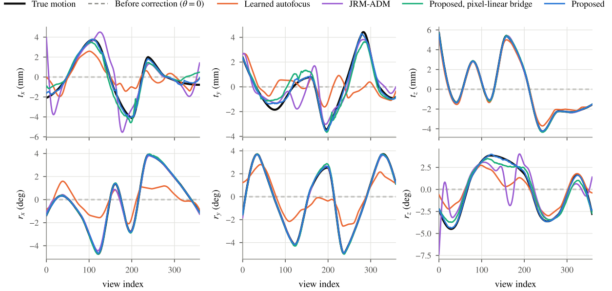
Figure 6: Recovered motion of one test patient (the first case of Fig. 5). Each panel shows one degree of freedom against the view index: the true trajectory, the state before correction ( \theta = 0 ), and the trajectory recovered by each method, all on the zero-mean gauge. Translations in mm, rotations in degrees.
