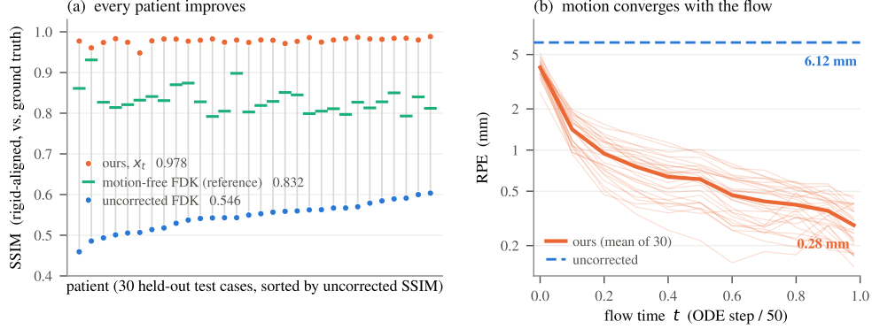
Figure 4: Cohort results over 30 held-out patients. (a) Per-patient SSIM; grey stems join each patient’s uncorrected and corrected score. (b) Reprojection error against flow time (thin: individual patients).
