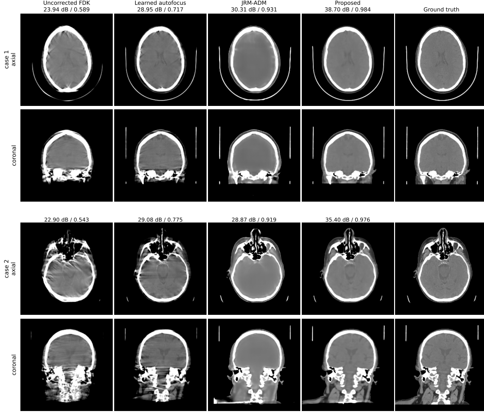
Figure 5: Qualitative comparison on two representative test patients, axial and coronal slices in the brain window; the axial slice of the second case lies at the skull-base level. All volumes are rigidly aligned to the ground truth before slicing, and labels give PSNR/SSIM against the ground truth.
