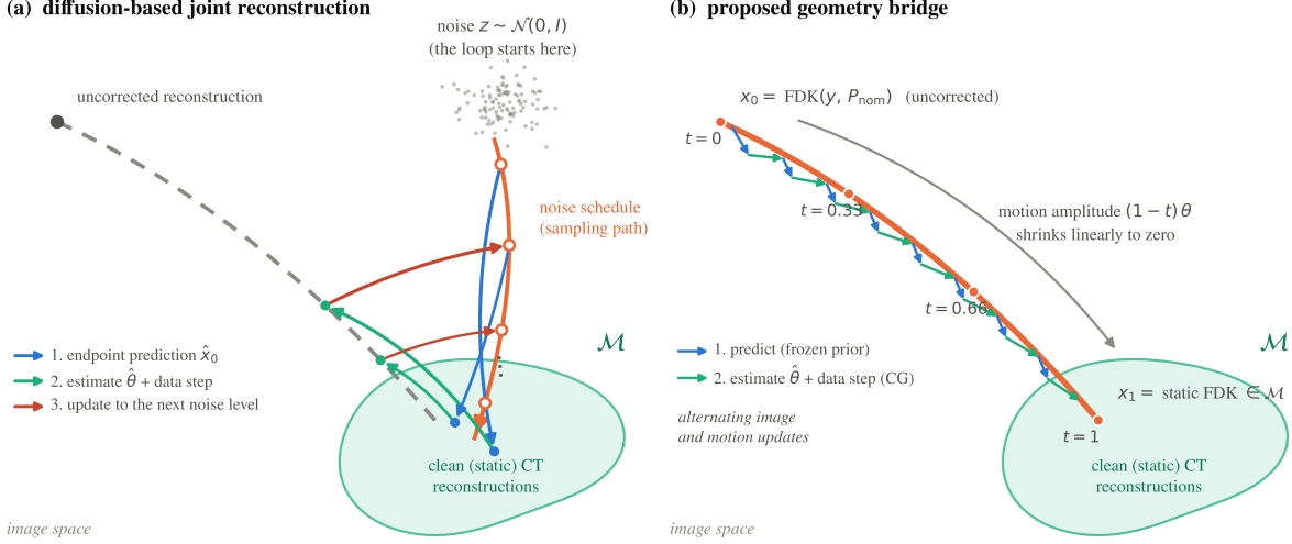
Figure 1: Schematic comparison of training paths and their use in joint reconstruction. (a) A noise-to-clean diffusion prior predicts an image that is combined with motion and data-consistency updates before advancing the sampling schedule. (b) The geometry bridge consists of FDK reconstructions simulated with motion amplitude (1 - t)\theta ; its tangent dx_t/dt is the training target. The learned velocity guides image updates interleaved with motion fitting and data consistency. The arrows illustrate the update sequence, not measured inference trajectories or projection onto the training bridge.
