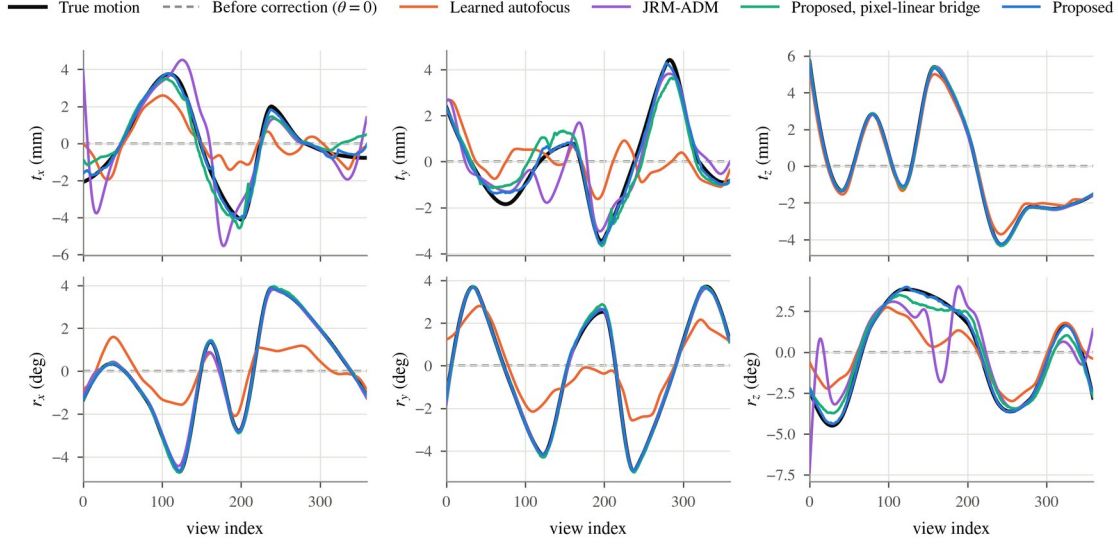
Figure 6: Recovered motion of one test patient (the first case of Fig. 5). Each panel shows one degree of freedom against the view index: the true trajectory, the state before correction ( \theta=0 ), and the trajectory recovered by each method, all on the zero-mean gauge. Translations in mm, rotations in degrees.
