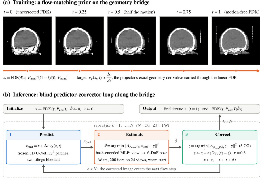
Figure 2: Training and inference. (a) FDK reconstructions of one volume re-simulated with motion amplitude (1-t)\theta . The training target is the path tangent, obtained by applying the fixed-geometry FDK operator to the projection derivative. (b) At inference, the frozen prior predicts an image, the motion estimator fits the measured projections to that prediction, and data consistency updates the image at the estimated geometry.
