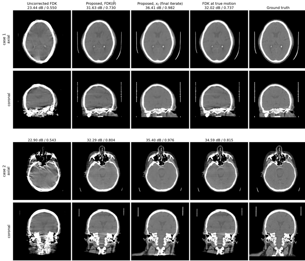
Figure 3: Two representative test patients at 10 mm/10° motion, brain window (level 40 / width 420 HU); volumes are rigidly aligned to the ground truth before display, and labels give PSNR/SSIM against the ground-truth volume. The fourth column is the FDK of the same scan at the true motion.
