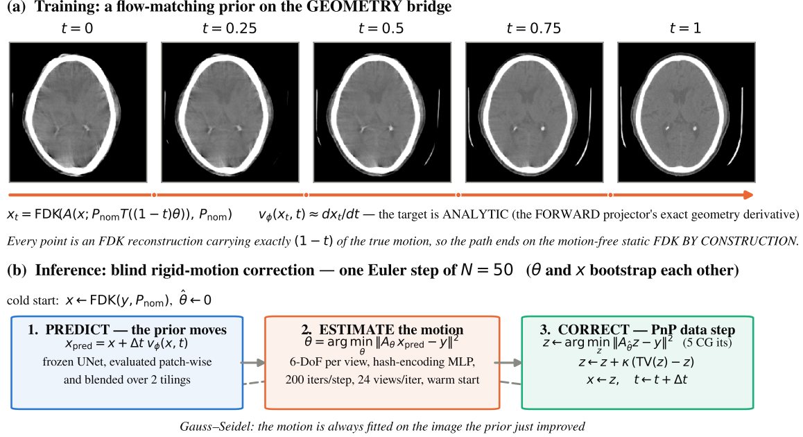
Figure 2: (a) The geometry bridge: each panel is an actual FDK reconstruction of a scan re-simulated with exactly (1-t) of the true motion, so the path ends on the motion-free static FDK by construction. The velocity target dx_t/dt is the forward projector’s exact geometry derivative carried through the linear FDK. (b) One step of the blind inference loop: the frozen prior moves the image, the motion is refit on the improved image, and a plug-and-play data step enforces consistency at the new estimate.
