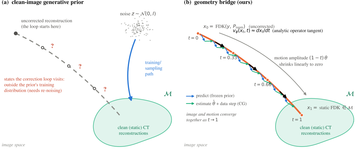
Figure 1: Concept of the proposed method. (a) A generative prior of clean images transports Gaussian noise to the clean-reconstruction manifold \mathcal{M} along a fixed path; the partially corrected reconstructions that a blind correction loop actually visits lie outside its training distribution and can only be reached through re-noising heuristics. (b) The geometry bridge makes that family of states the training path itself: x_t is the FDK reconstruction of the same scan carrying (1-t) of the motion, the path ends on the static FDK by construction, and the regression target is the analytic operator tangent dx_t/dt . Inference walks the bridge: the frozen prior advances the image along the learned velocity, the motion is refit on the improved image, and the data-consistency step returns the iterate to the bridge, so the image and the motion converge together as t \rightarrow 1 .
