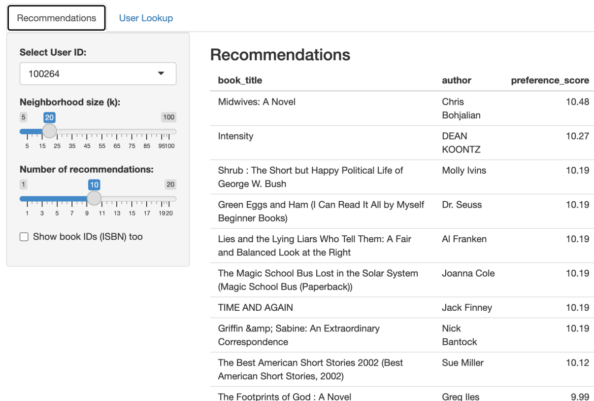
Figure 2: Figure illustrates the Recommendations tab, where users can adjust neighborhood size and number of recommendations
