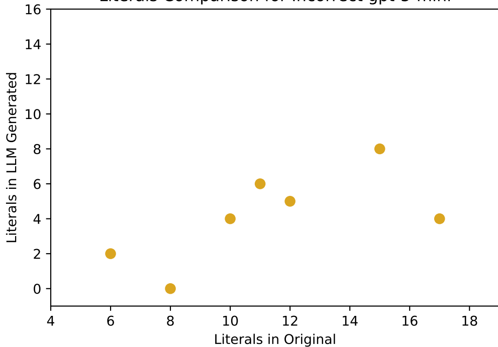
Literals Comparison for Incorrect gpt-5-mini
