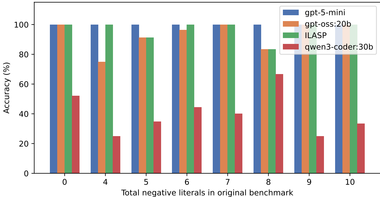
Accuracy by negative literal count
