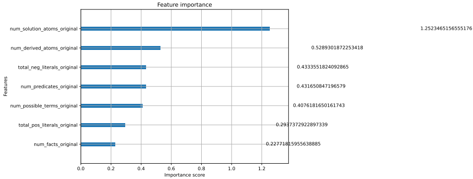
Figure 8: XGBoost feature importance of ASP features predicting LLM success.
