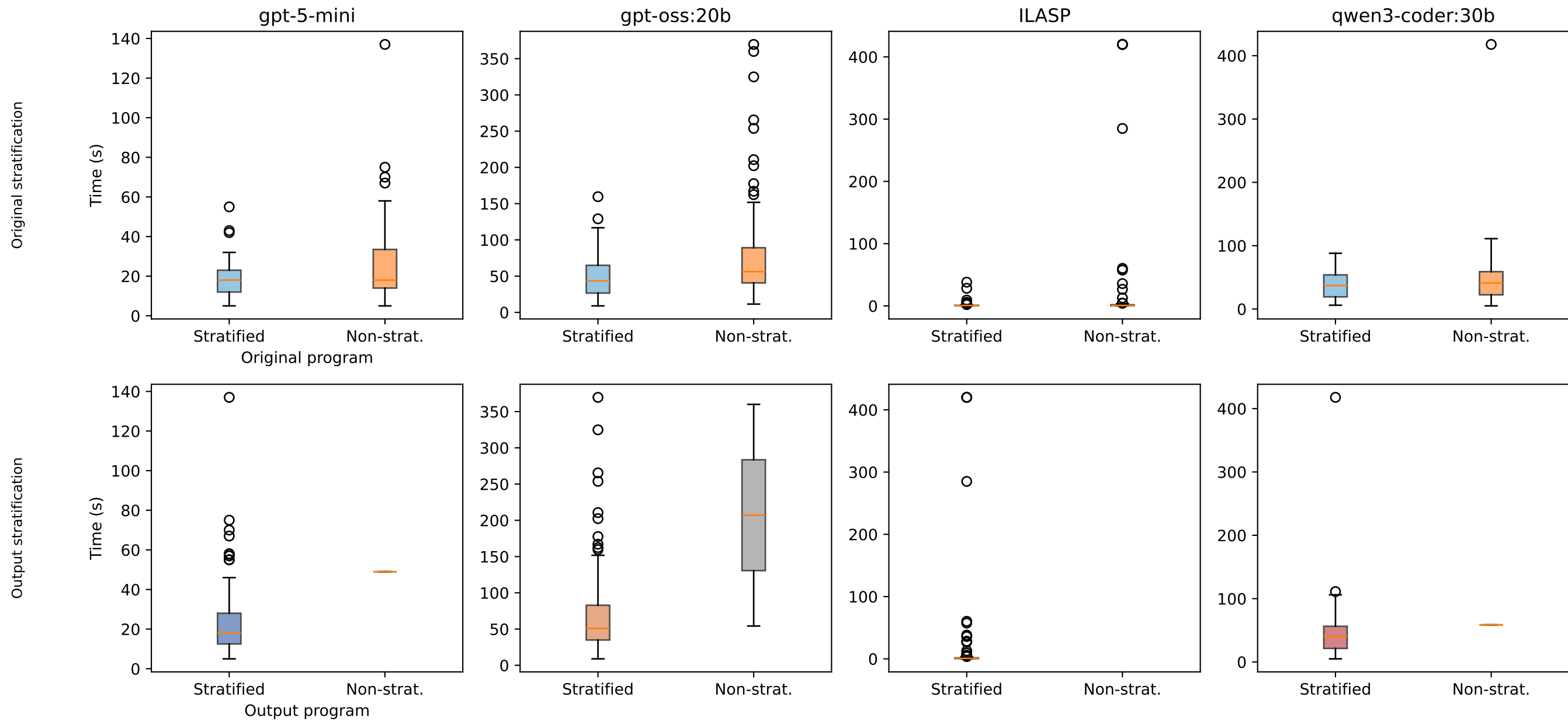
Time to solve by stratification (original vs. output)
