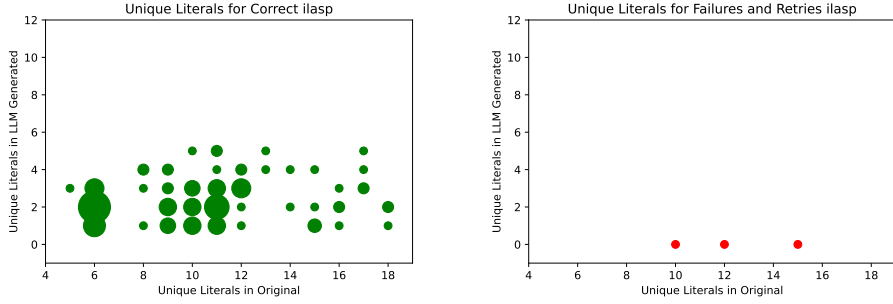
Figure 7: ILASP unique literal counts (timed out in red on right).
