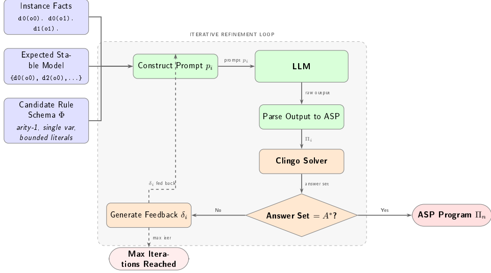
Figure 1: Overview of the LAMP pipeline.
