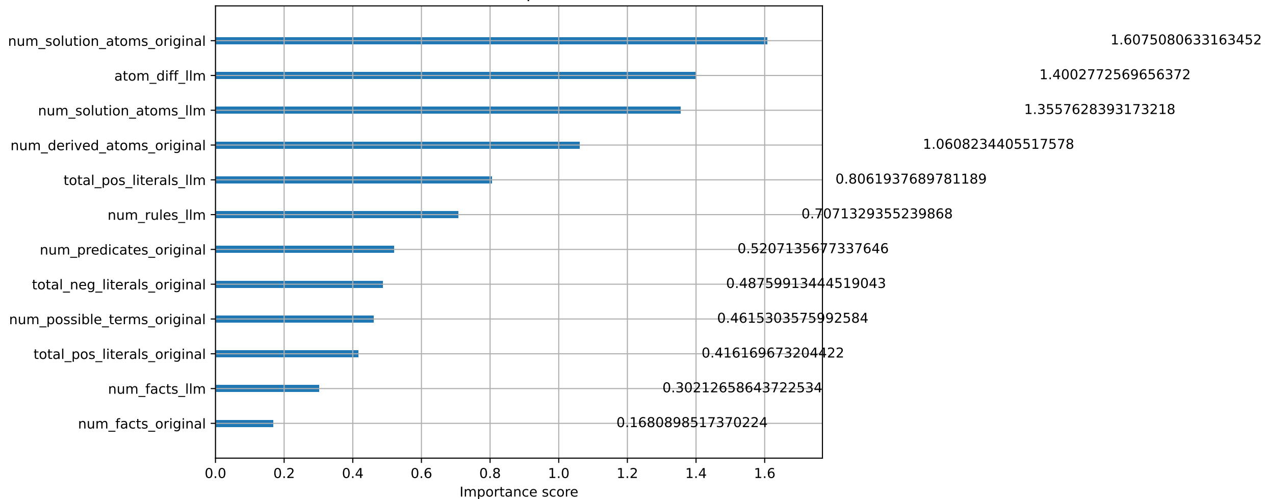
Feature importance
