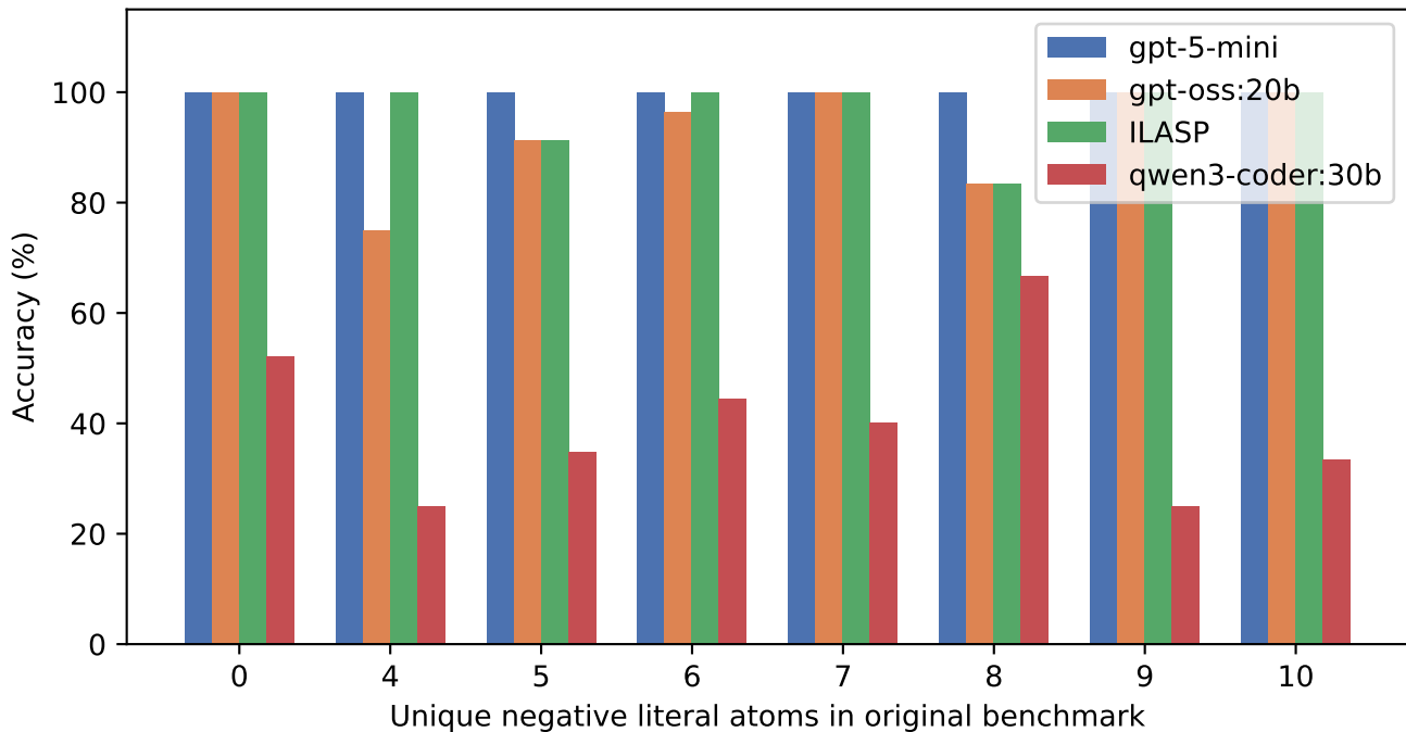
Accuracy by unique negative literal atom count
