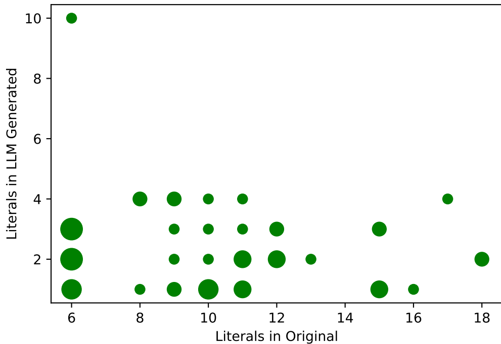
Literals Comparison for Correct qwen3-coder:30b
