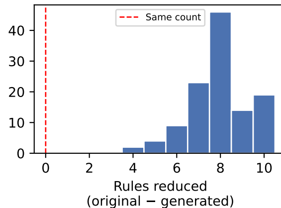
ILASP
