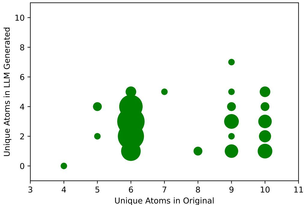
Unique Atoms Comparison for Correct gpt-5-mini
