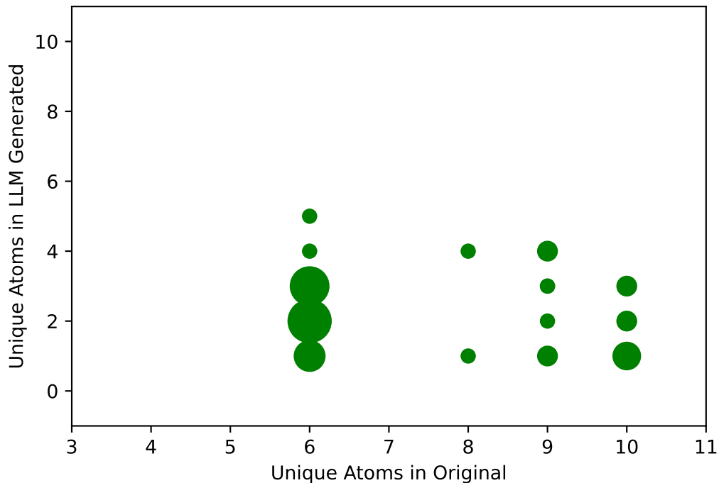
Unique Atoms Comparison for Correct qwen3-coder:30b
