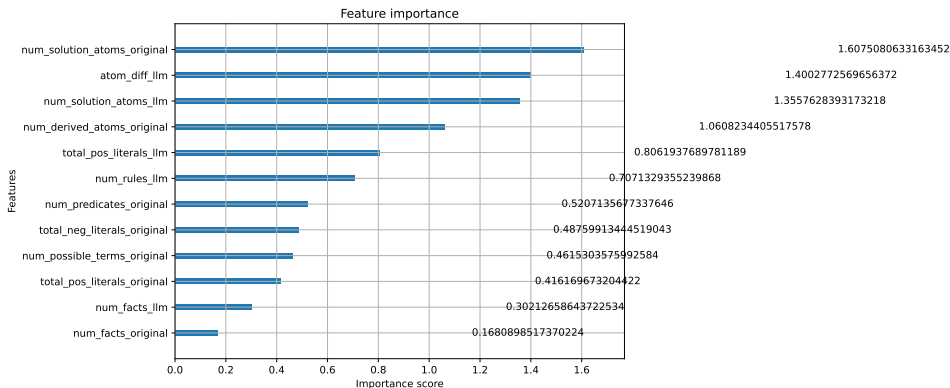
Figure 8: XGBoost Feature Importance
