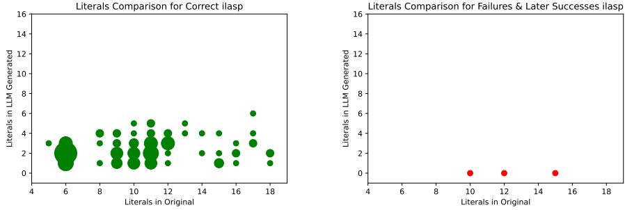
Figure 7: Qwen3-coder input literals to output literals for correct answer set response.
