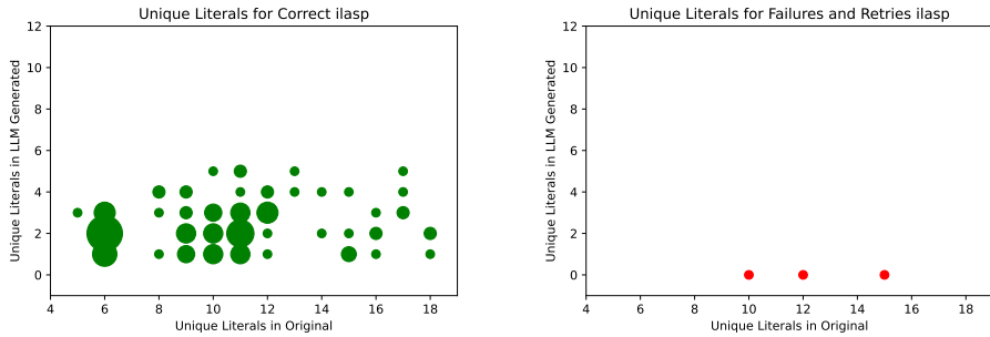
Figure 7: ILASP unique literal counts (correct on left, timed out in red on right).
