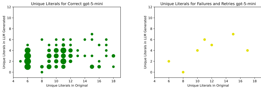
Figure 4: Unique literal counts for gpt-5-mini (correct on left, recovered in gold and failed in red on right).
