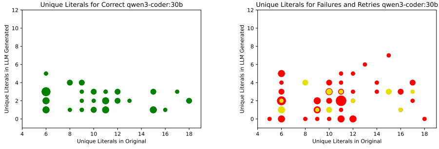
Figure 6: Unique literal counts for qwen3-coder:30b (correct on left, recovered in gold and failed in red on right).
