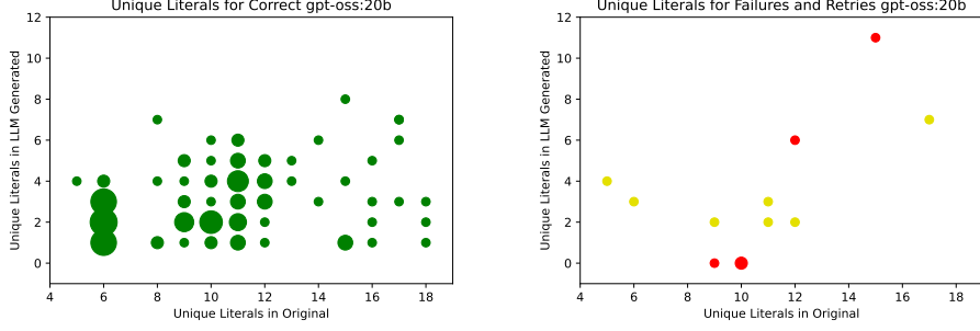
Figure 5: Unique literal counts for gpt-oss:20b (correct on left, recovered in gold and failed in red on right).
