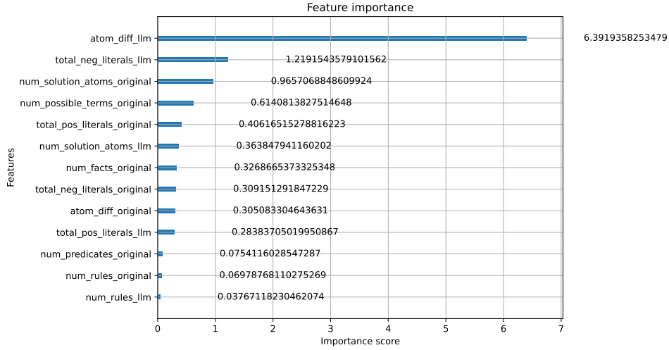
Figure 5: XGBoost Feature Importance
