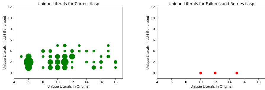
Figure 7: ILASP unique literal counts (correct on left, timed out in red on right).
