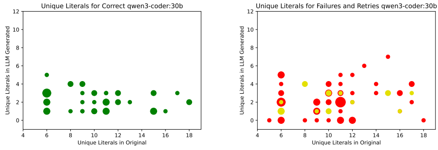
Figure 6: Unique literal counts for qwen3-coder:30b (correct on left, recovered in gold and failed in red on right).
