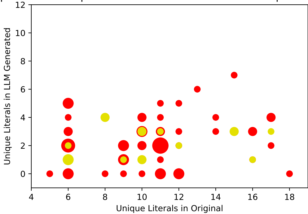
Unique Literals Comparison for Failures & Later Successes qwen3-coder:3
