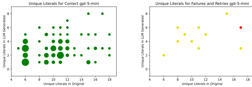
Figure 4: Unique literal counts for gpt-5-mini .
