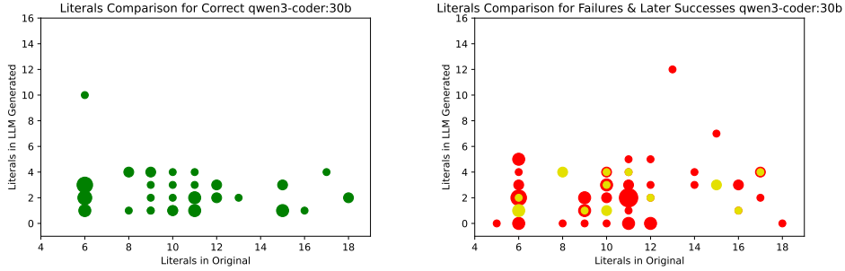
Figure 6: Qwen3-coder:30b literal counts (left: correct, right: recovered (gold) / failed (red)).
