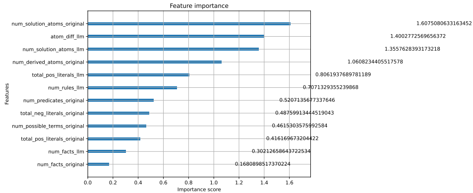
Figure 8: XGBoost feature importance of ASP features predicting LLM success.
