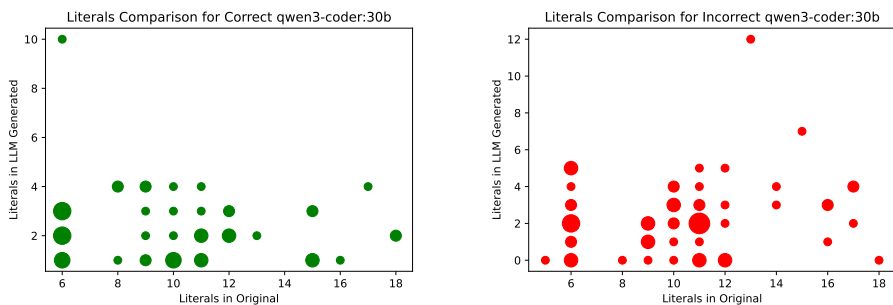
Figure 4: Qwen3-coder input literals to output literals for correct answer set response.
