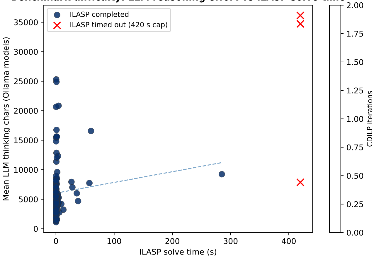
Benchmark difficulty: LLM reasoning effort vs ILASP solve time
