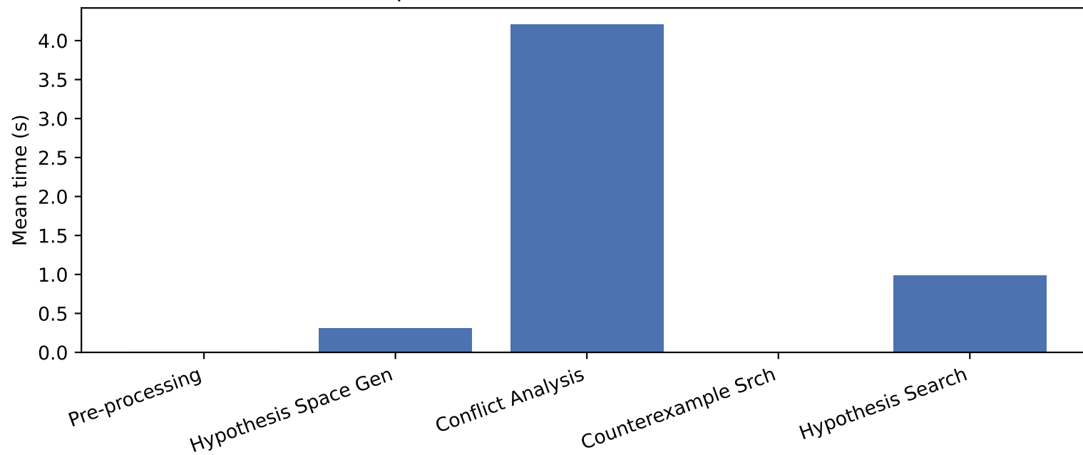
ILASP phase times (non-timeout benchmarks)
