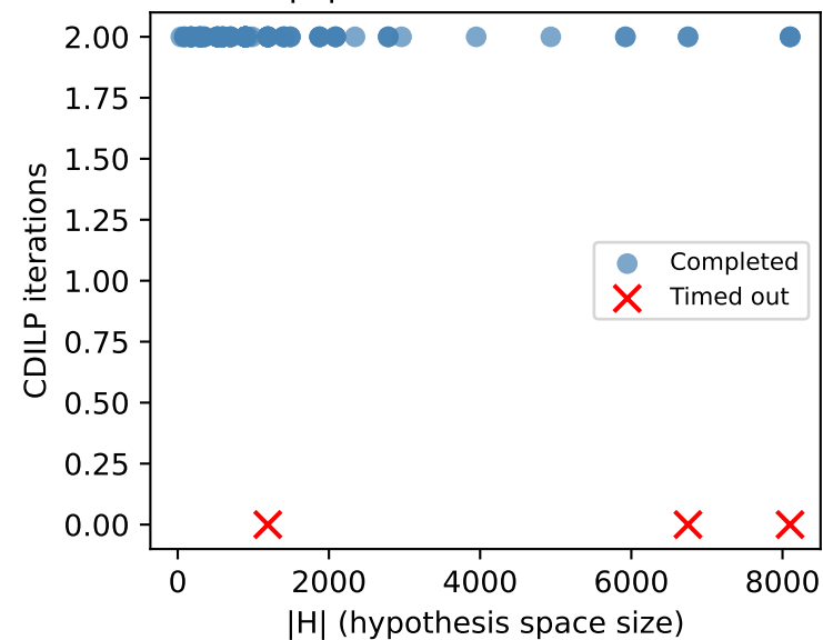
|H| vs CDILP iterations
