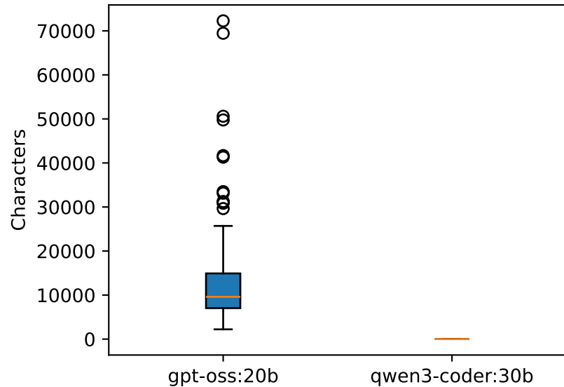
Thinking chars (Ollama)
