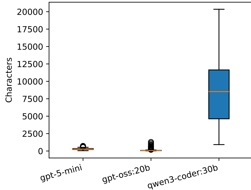
Content chars (all models)
