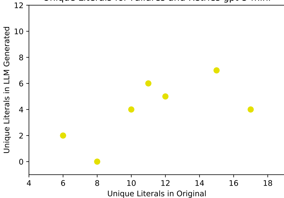
Unique Literals for Failures and Retries gpt-5-mini
