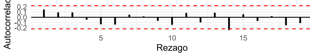
Correlograma PACF
