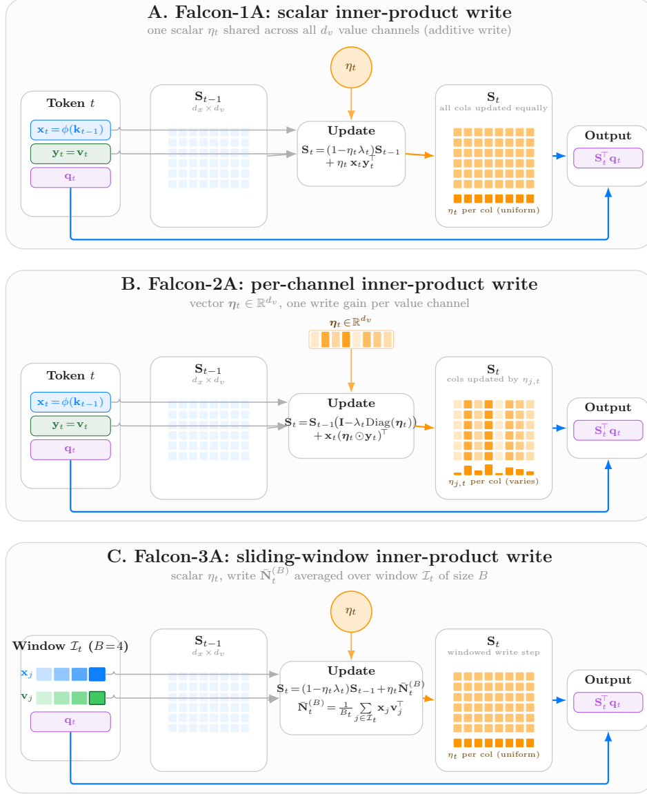
Figure 6 Falcon-1A vs. Falcon-2A vs. Falcon-3A. Each panel shows one inner-product fast-weight update step on the fixed-size state \mathbf{S}_{t-1} \in \mathbb{R}^{d_x \times d_v} . We write \mathbf{q}_t := \phi(\mathbf{q}_t) for the query feature. Unlike the regression family (Falcon-1/2/3), these rules write the target directly rather than a residual: there is no \mathbf{S}_{t-1}^\top \mathbf{x}_t subtraction inside the write. Forgetting acts only on the carry—through a scalar factor in Falcon-1A/Falcon-3A and through per-column factors in Falcon-2A. (A) Falcon-1A applies one scalar \eta_t to all d_v value channels; every column of \mathbf{S}_t receives the same energy-normalized write gain \eta_t = \beta_t / (\|\mathbf{x}_t\|_2^2 + \lambda_t + \varepsilon) (uniform orange shading and flat per-column bar). (B) Falcon-2A promotes the write gain to a vector \eta_t \in \mathbb{R}^{d_v} shown as the orange strip above the update card: each column of \mathbf{S}_t receives its own gain \eta_{j,t} , while the write feature \mathbf{x}_t and target \mathbf{v}_t remain shared. (C) Falcon-3A returns to a scalar \eta_t but writes the windowed average cross-covariance \tilde{\mathbf{N}}_t^{(B)} = B_t^{-1} \sum_{j \in \mathcal{I}_t} \mathbf{x}_j \mathbf{v}_j^\top over a sliding window \mathcal{I}_t of B recent causal pairs; the blue/green strips show four \{\mathbf{x}_j, \mathbf{v}_j\}_{j \in \mathcal{I}_t} entries. The denominator \eta_t = \beta_t / (\bar{E}_t^{(B)} + \lambda_t + \varepsilon) uses the window energy \bar{E}_t^{(B)} as a write-magnitude normalizer. The read \mathbf{o}_t = \mathbf{S}_t^\top \mathbf{q}_t uses the updated state in all three cases.
