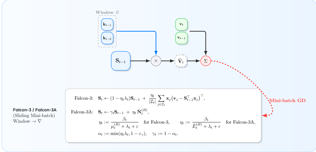
Figure 3 Conceptual Overview. (A) Many fast-weight rules bind the same-step write-feature/target pair (\phi(\mathbf{k}_t), \mathbf{v}_t) as a cache-style association. Under the prefix-prediction fast-memory objective studied here, the example revealed at step t pairs a prefix write feature with the newly observed target, yielding (\phi(\mathbf{k}_{t-1}), \mathbf{v}_t) . (B) Falcon-1 / Falcon-2 (Next-Latent Prediction) : the state \mathbf{S}_{t-1} predicts \mathbf{v}_t from the prefix feature \mathbf{x}_t := \phi(\mathbf{k}_{t-1}) , then performs an online NLMS-stabilized ridge-regression update. (C) Falcon-3 / Falcon-3A (Sliding Mini-batch) : applies a mini-batch regression (or inner-product) step over an active window \mathcal{I}_t of nominal size B (realized size B_t := |\mathcal{I}_t| \leq B ) over causal pairs (\mathbf{x}_j, \mathbf{v}_j) with \mathbf{x}_j := \phi(\mathbf{k}_{j-1}) .
