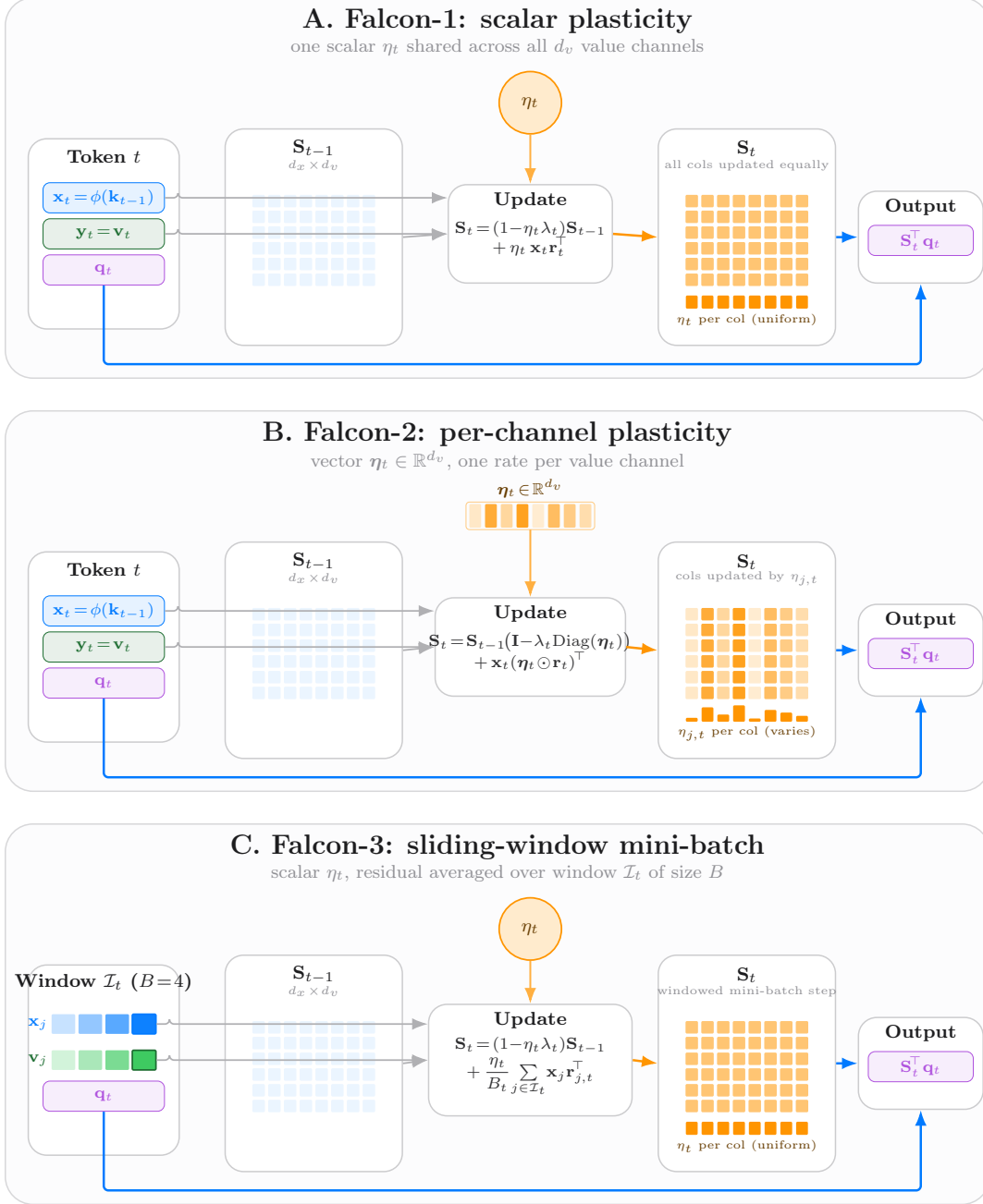
Figure 1 Falcon-1 vs. Falcon-2 vs. Falcon-3. Each panel shows one fast-weight update step on the fixed-size matrix state \mathbf{S}_{t-1} \in \mathbb{R}^{d_x \times d_v} . We write \mathbf{q}_t := \phi(\mathbf{q}_t) for the query feature. In panels (A)–(B), \mathbf{r}_t := \mathbf{v}_t - \mathbf{S}_{t-1}^\top \mathbf{x}_t . (A) Falcon-1 applies one scalar \eta_t to all d_v value channels; every column of \mathbf{S}_t receives the same plasticity. (B) Falcon-2 promotes the step size to a vector \eta_t \in \mathbb{R}^{d_v} shown as the orange strip above the update card: each column of \mathbf{S}_t is updated with its own gain \eta_{j,t} , while the write feature \mathbf{x}_t and residual \mathbf{r}_t remain shared. (C) Falcon-3 uses a scalar \eta_t and a sliding window \mathcal{I}_t of B recent causal pairs, with window residuals \mathbf{r}_{j,t} := \mathbf{v}_j - \mathbf{S}_{t-1}^\top \mathbf{x}_j ; the blue/green strips show four \{\mathbf{x}_j, \mathbf{v}_j\}_{j \in \mathcal{I}_t} entries. The read \mathbf{o}_t = \mathbf{S}_t^\top \mathbf{q}_t uses the updated state in all three cases.
