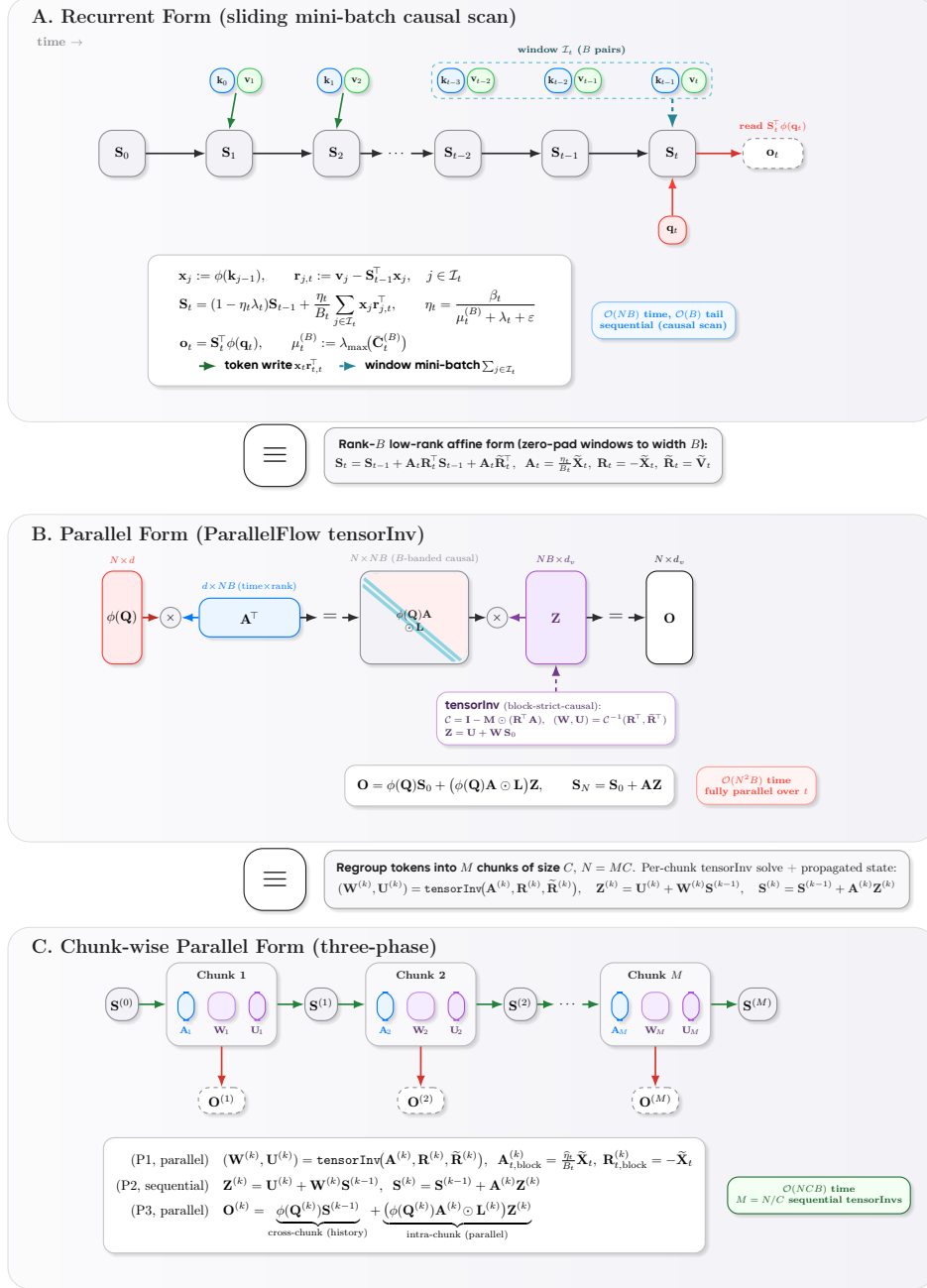
Figure 9 Three equivalent views of Falcon-3. (A) The recurrent form maintains a fixed-size matrix state \mathbf{S}_t \in \mathbb{R}^{d_x \times d_v} . Each step writes a mini-batch gradient on the window \mathcal{I}_t of the last B causal pairs \{(\phi(\mathbf{k}_{j-1}), \mathbf{v}_j)\}_{j \in \mathcal{I}_t} , with all residuals \mathbf{r}_{j,t} = \mathbf{v}_j - \mathbf{S}_{t-1}^\top \mathbf{x}_j evaluated at the pre-update state. (B) After the scalar positive-decay renormalization (the identity when \lambda_t = 0 ), zero-padding each active window to width B recasts the update as a rank- B affine recurrence \mathbf{S}_t = \mathbf{S}_{t-1} + \mathbf{A}_t \mathbf{R}_t^\top \mathbf{S}_{t-1} + \mathbf{A}_t \tilde{\mathbf{R}}_t^\top . (C) Splitting the sequence into M chunks of size C yields the exact three-phase ParallelFlow algorithm.
