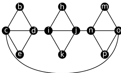
Figure 12.147 Graph G
