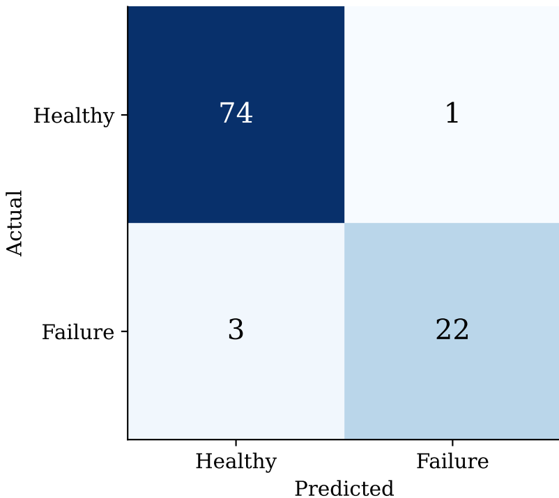
Confusion matrix (thr = 0.780)
