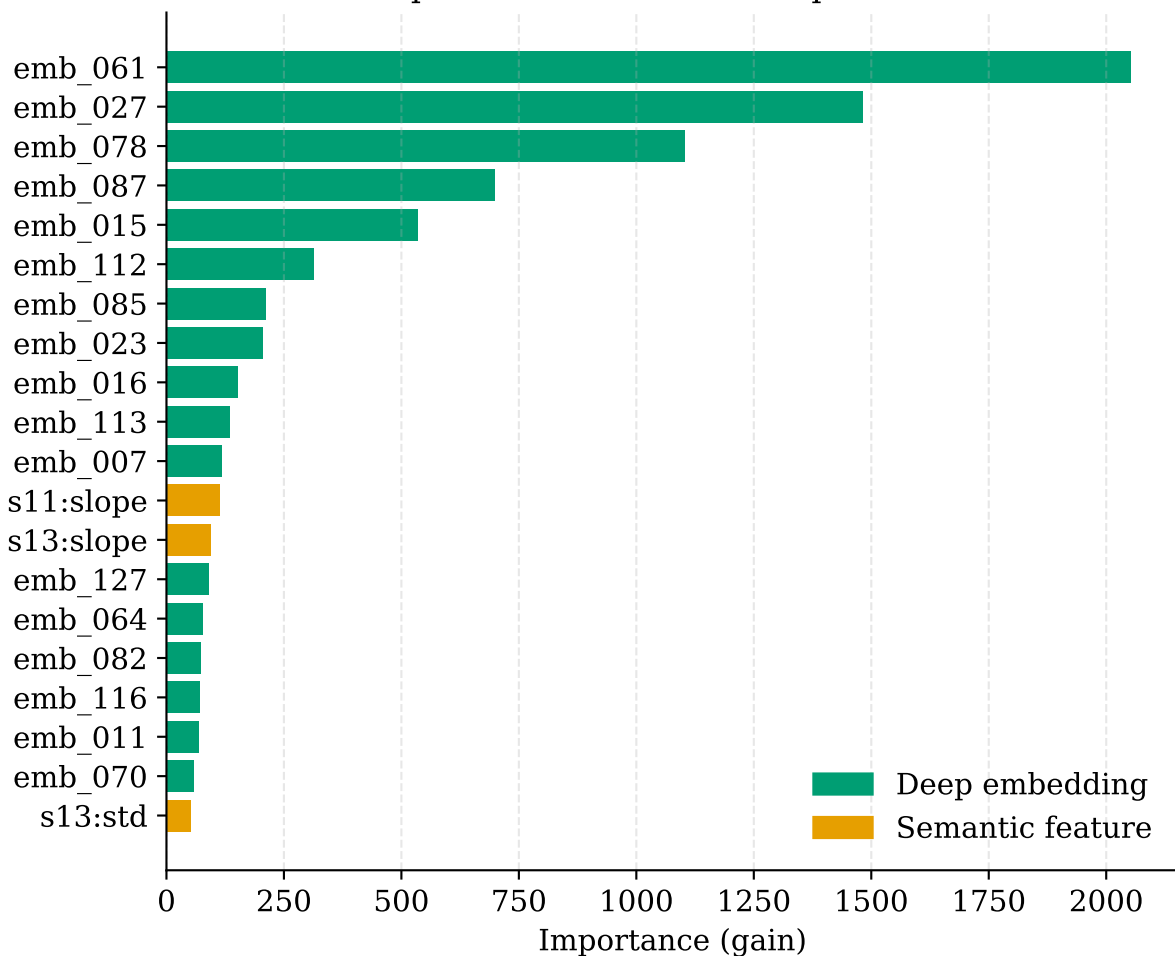
Top-20 XGBoost feature importances
