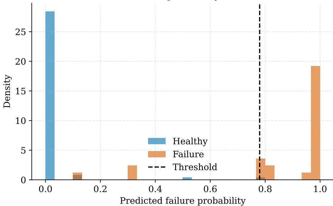
Class-conditional probability distributions
