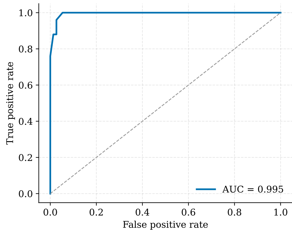
ROC curve
