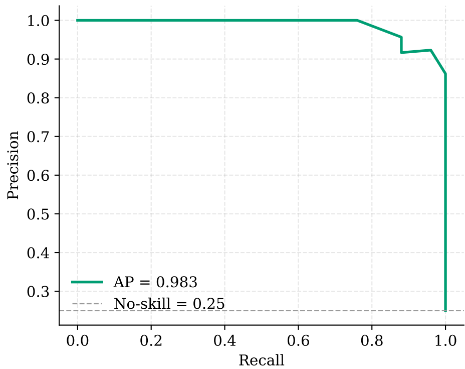
Precision-Recall curve
