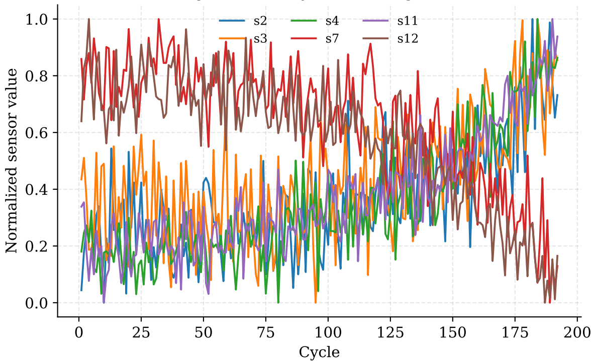
Sensor degradation trajectories (engine 1, FD001)
