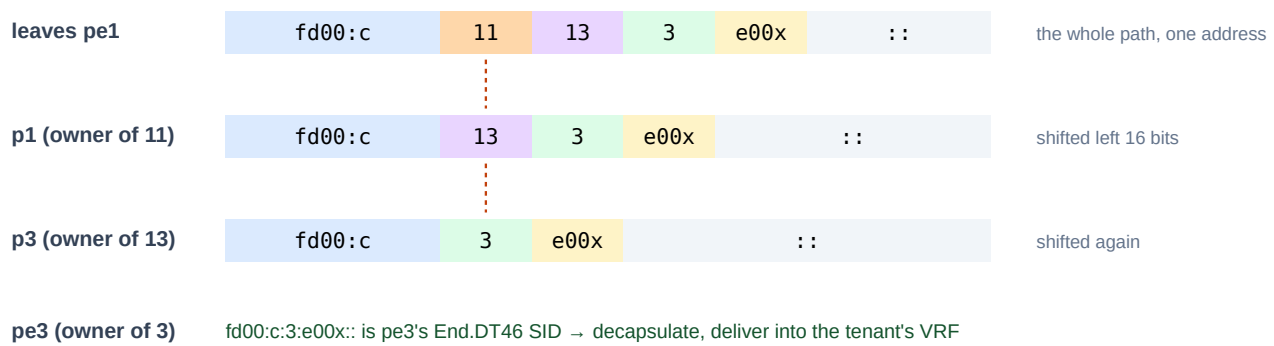
Figure 5 — the steered path pe1 \rightarrow p1 \rightarrow p3 \rightarrow pe3 as a single uSID "carrier" (Part 3, step 8, shows these three addresses on the wire).
