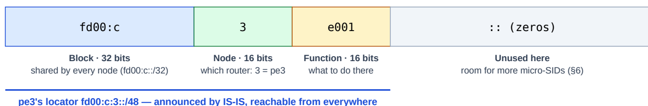
Figure 2 — the SID fd00:c:3:e001:: read as an instruction: "go to pe3, and there apply function e001" (in this lab: hand the packet to one tenant's routing table).
