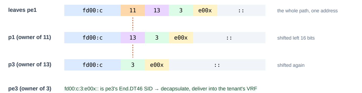
Figure 5 — the steered path pe1 → p1 → p3 → pe3 as a single uSID "carrier" (Part 3, step 8, shows these three addresses on the wire).
