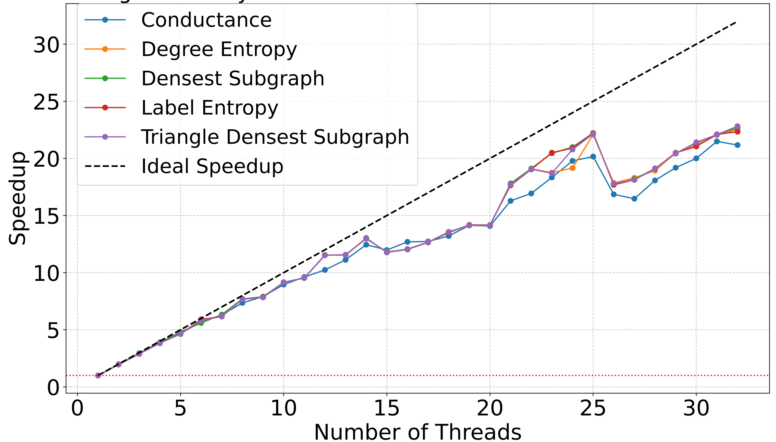
Strong Scalability for Citeseer with VNS Run Timeout of 1 seconds
