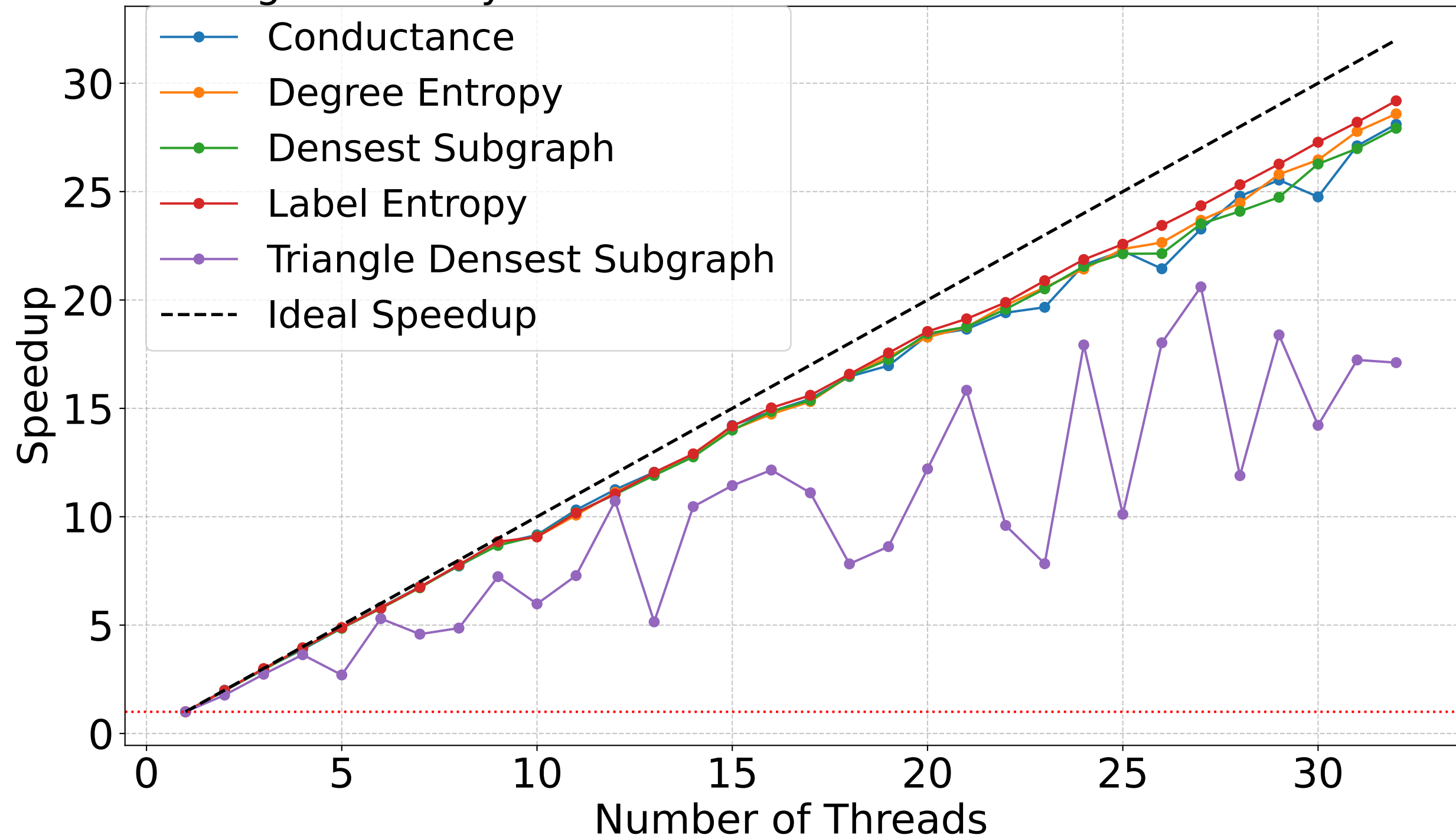
Strong Scalability for DBLP with VNS Run Timeout of 3 seconds
