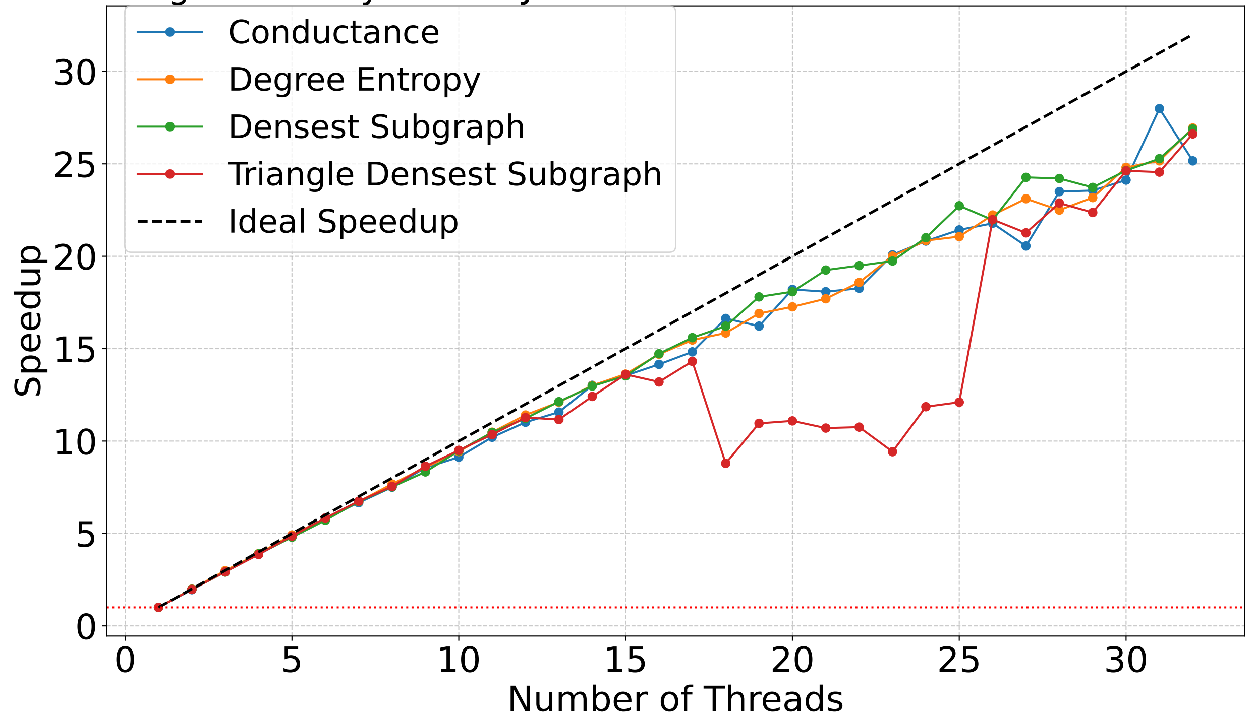
Strong Scalability for LiveJournal with VNS Run Timeout of 3 second
