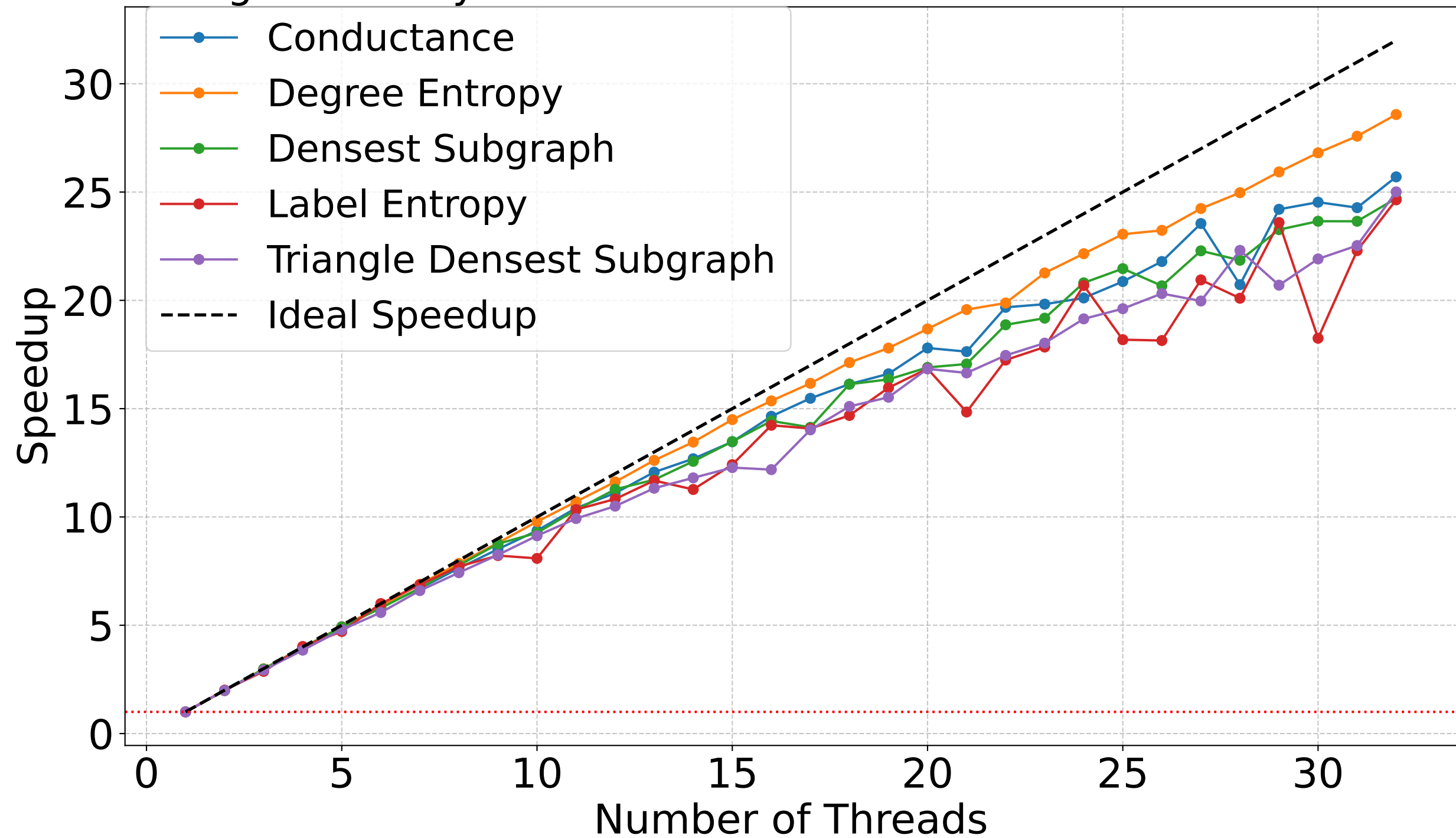
Strong Scalability for Youtube with VNS Run Timeout of 1 seconds
